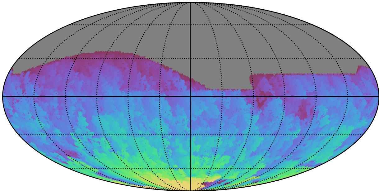
too_elab_r32_d3_ugrizy_v3.4_10yrs All sky r band: Max HA
