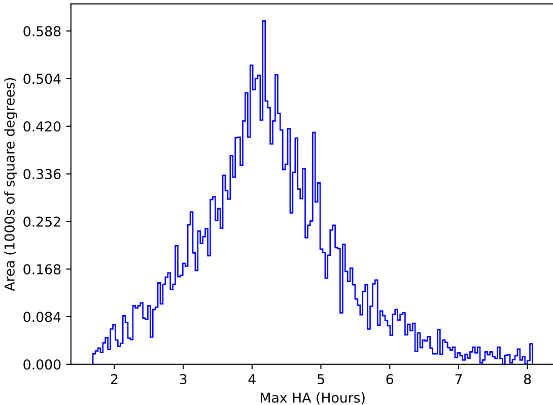
too_elab_r32_d3_ugrizy_v3.4_10yrs All sky r band: Max HA
