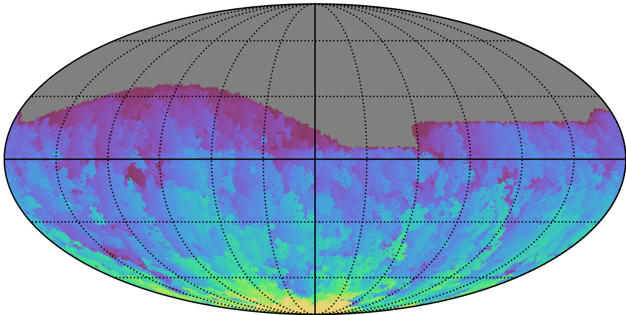
too_elab_r32_d3_ugrizy_v3.4_10yrs All sky g band: Max HA
