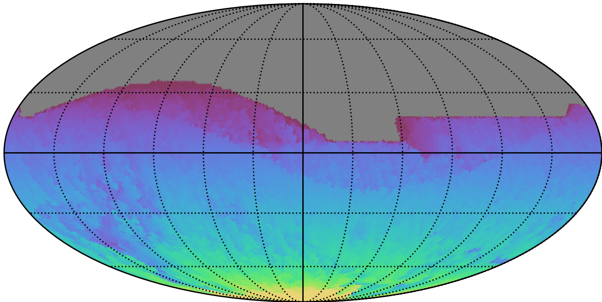
too_elab_r32_d3_ugrizy_v3.4_10yrs All sky all bands: Max HA
