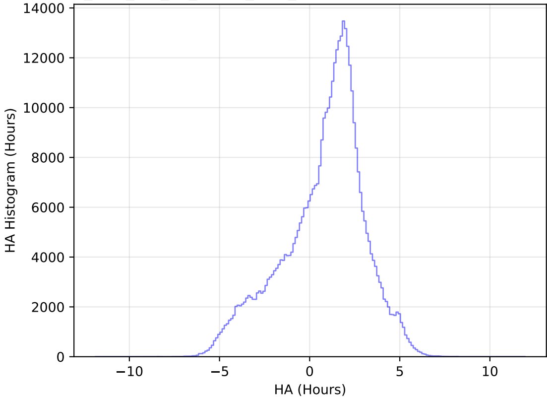
too_elab_r32_d3_ugrizy_v3.4_10yrs WFD z band: HA Histogram
