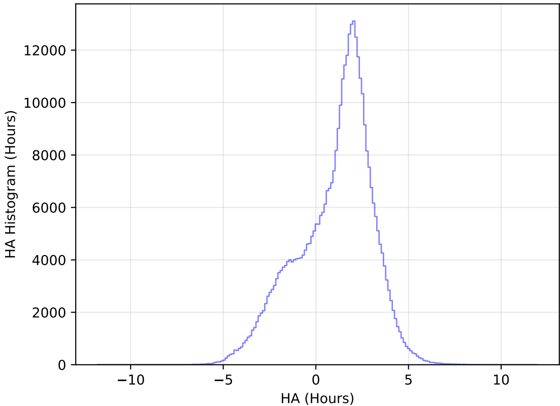
too_elab_r32_d3_ugrizy_v3.4_10yrs WFD y band: HA Histogram
