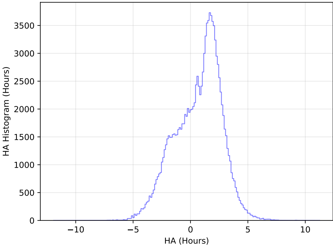
too_elab_r32_d3_ugrizy_v3.4_10yrs WFD u band: HA Histogram
