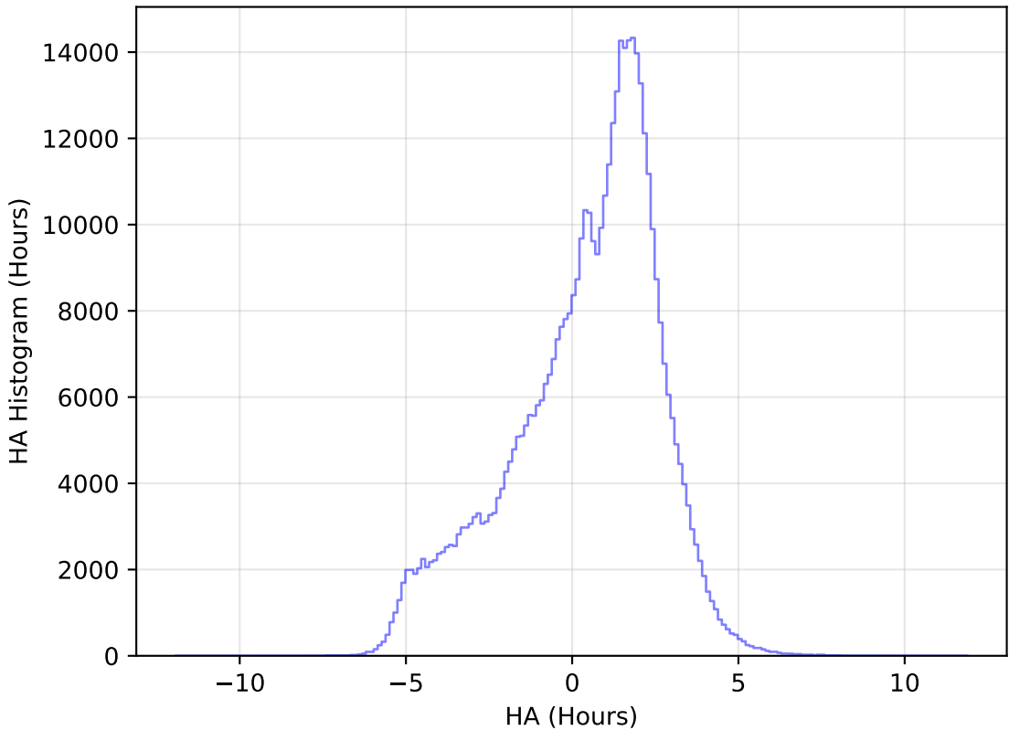
too_elab_r32_d3_ugrizy_v3.4_10yrs WFD r band: HA Histogram
