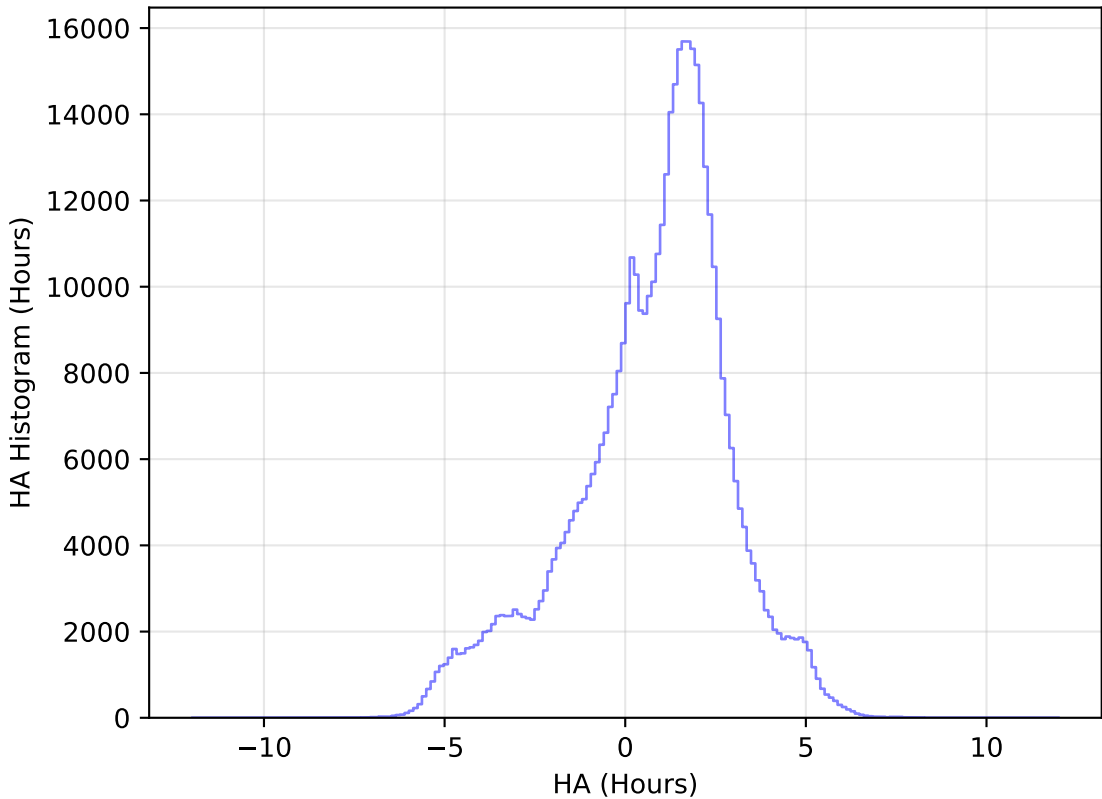
too_elab_r32_d3_ugrizy_v3.4_10yrs WFD i band: HA Histogram
