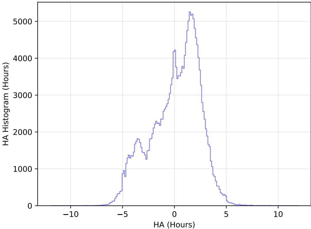
too_elab_r32_d3_ugrizy_v3.4_10yrs WFD g band: HA Histogram
