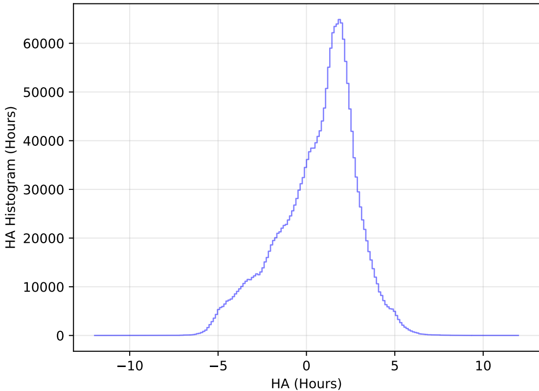
too_elab_r32_d3_ugrizy_v3.4_10yrs WFD all bands: HA Histogram
