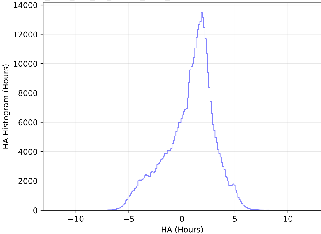
too_elab_r32_d3_ugrizy_v3.4_10yrs All sky z band: HA Histogram
