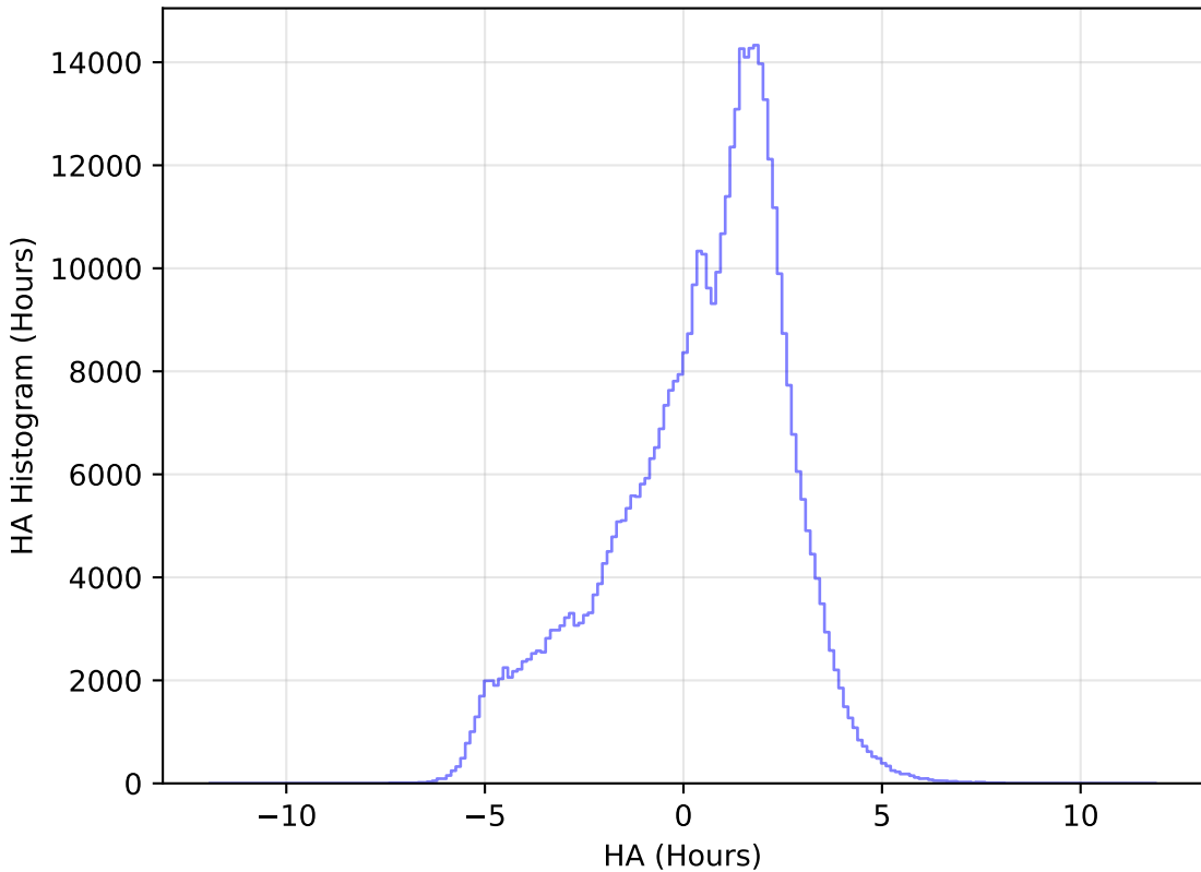
too_elab_r32_d3_ugrizy_v3.4_10yrs All sky r band: HA Histogram
