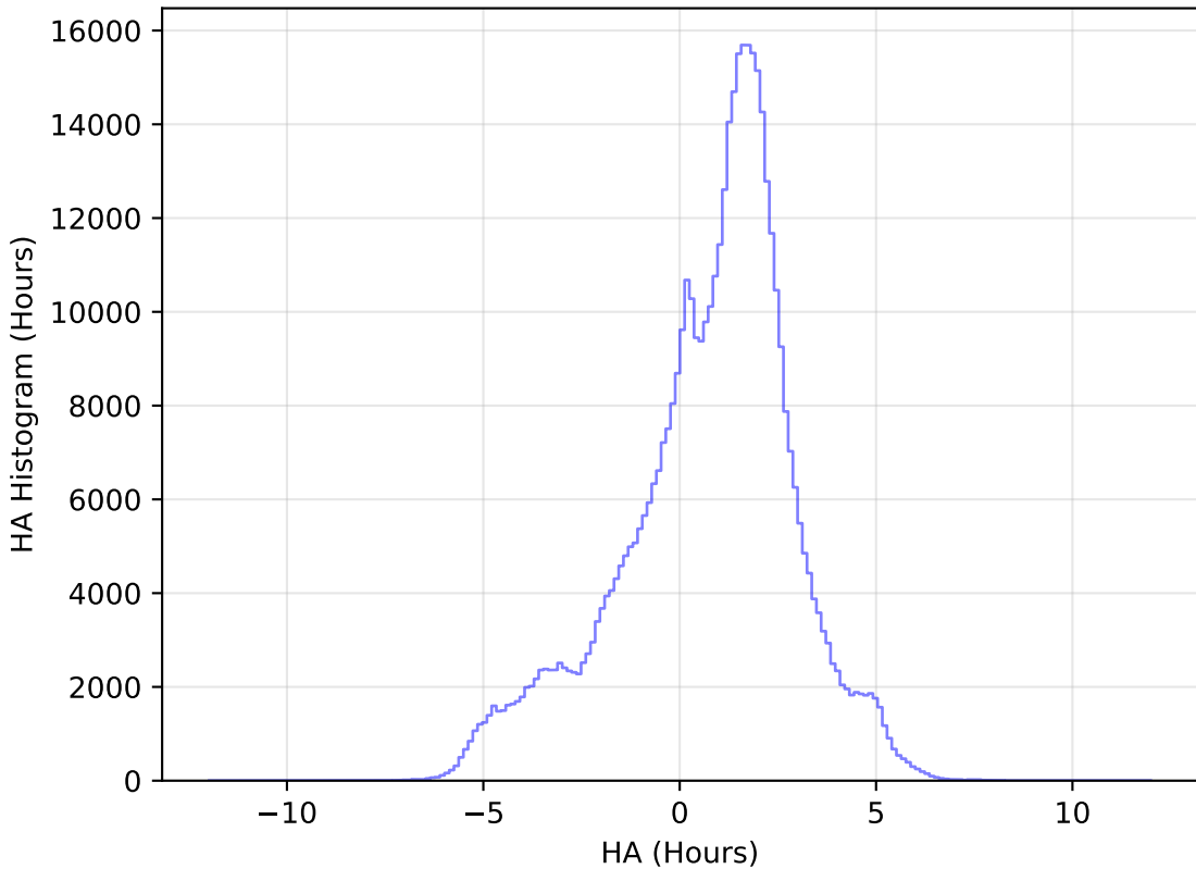
too_elab_r32_d3_ugrizy_v3.4_10yrs All sky i band: HA Histogram
