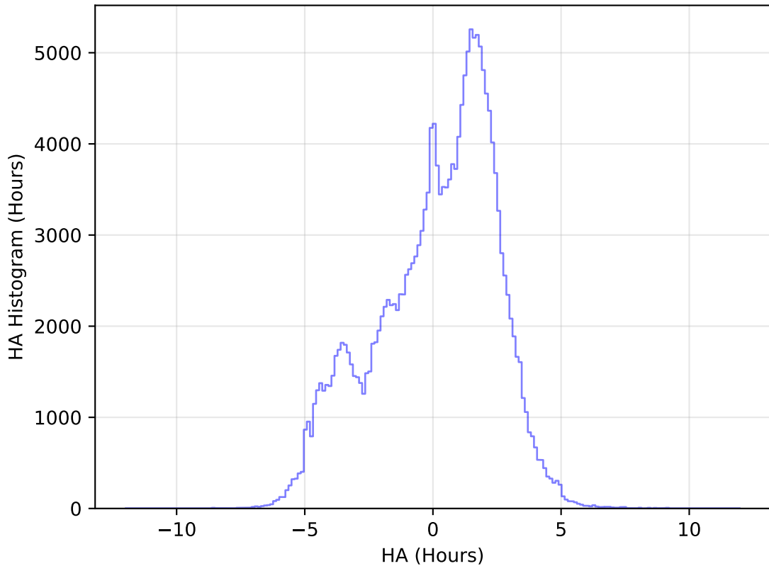
too_elab_r32_d3_ugrizy_v3.4_10yrs All sky g band: HA Histogram
