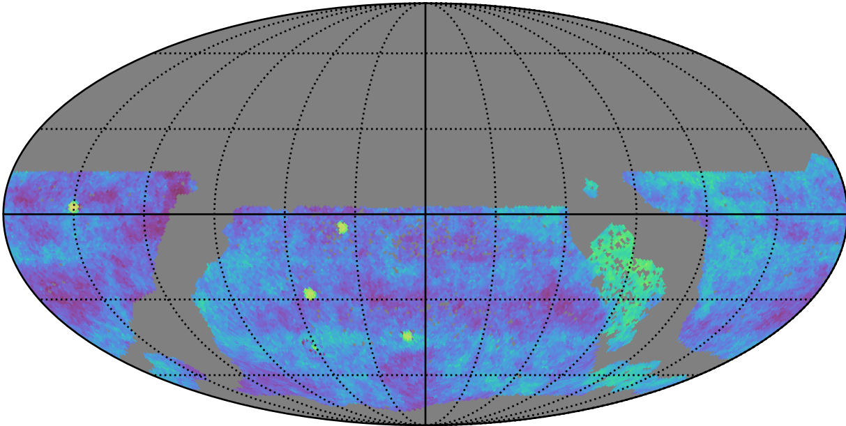
too_elab_r32_d3_ugrizy_v3.4_10yrs gri WFD: Fraction of visits in pairs (20-90 min)
