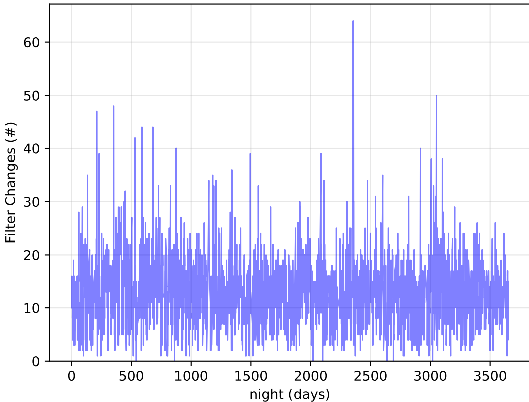
too_elab_r32_d3_ugrizy_v3.4_10yrs Per Night: Filter Changes
