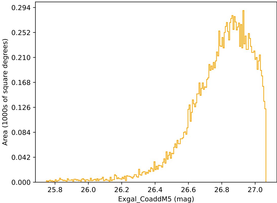
too_elab_r32_d3_ugrizy_v3.4_10yrs WFD r band: Exgal_CoaddM5
