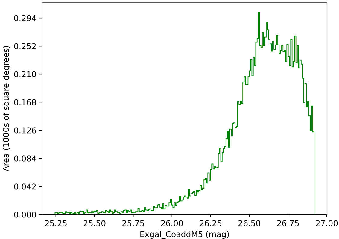
too_elab_r32_d3_ugrizy_v3.4_10yrs WFD g band: Exgal_CoaddM5
