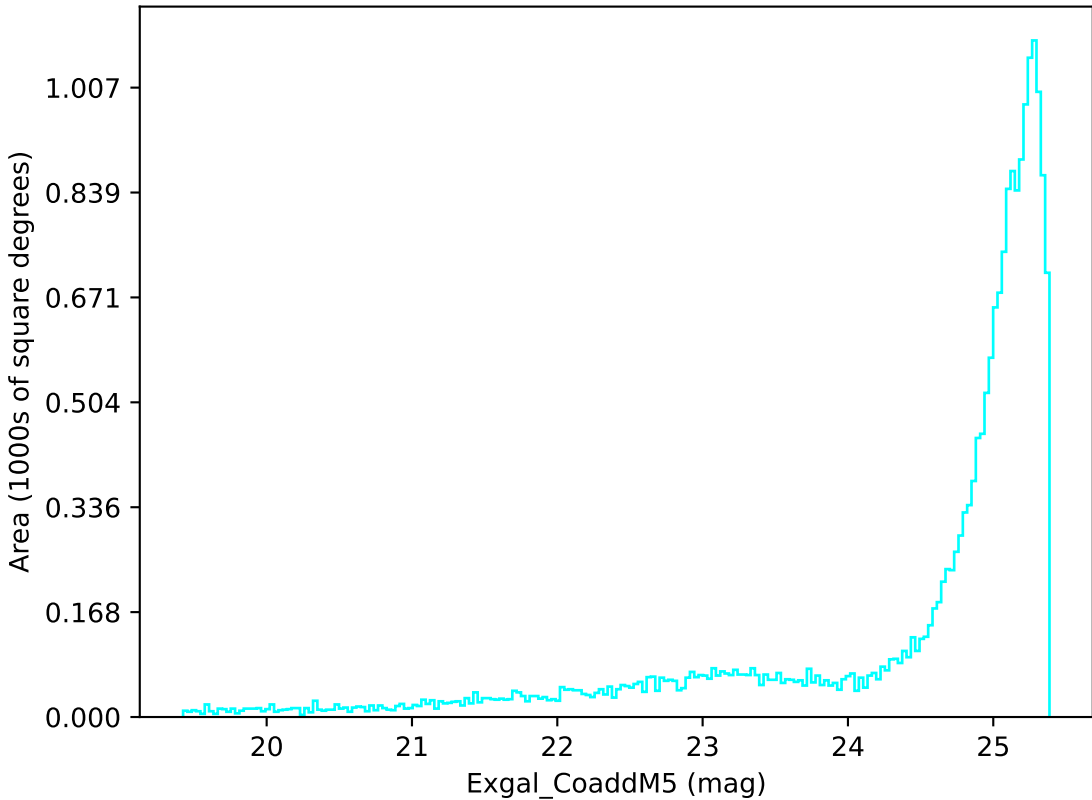
too_elab_r32_d3_ugrizy_v3.4_10yrs All sky u band: Exgal_CoaddM5
