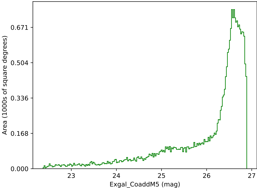
too_elab_r32_d3_ugrizy_v3.4_10yrs All sky g band: Exgal_CoaddM5
