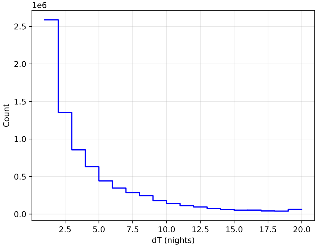
too_elab_r32_d3_ugrizy_v3.4_10yrs WFD all bands: DeltaNight Histogram
