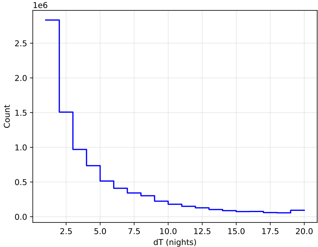
too_elab_r32_d3_ugrizy_v3.4_10yrs All sky all bands: DeltaNight Histogram
