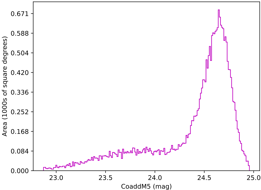
too_elab_r32_d3_ugrizy_v3.4_10yrs Yr 1 z band: CoaddM5
