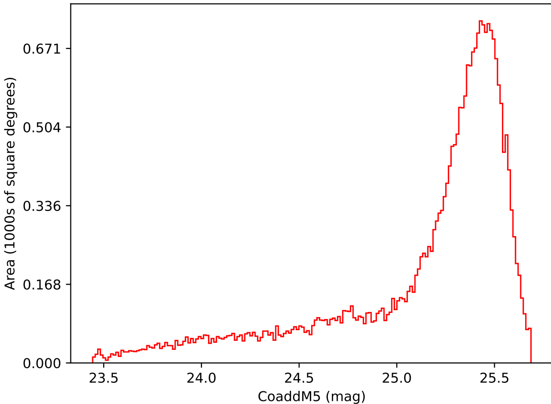
too_elab_r32_d3_ugrizy_v3.4_10yrs Yr 1 i band: CoaddM5
