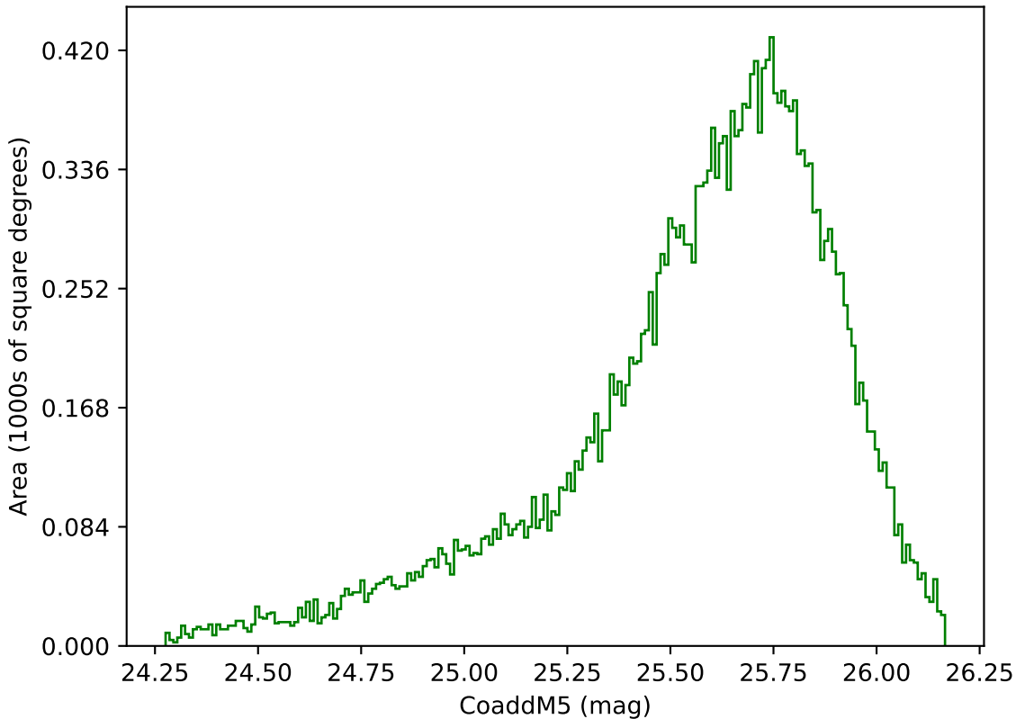
too_elab_r32_d3_ugrizy_v3.4_10yrs Yr 1 g band: CoaddM5
