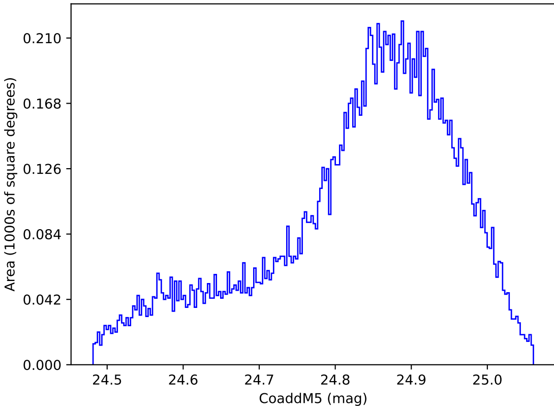
too_elab_r32_d3_ugrizy_v3.4_10yrs WFD y band: CoaddM5
