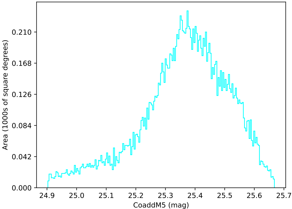
too_elab_r32_d3_ugrizy_v3.4_10yrs WFD u band: CoaddM5
