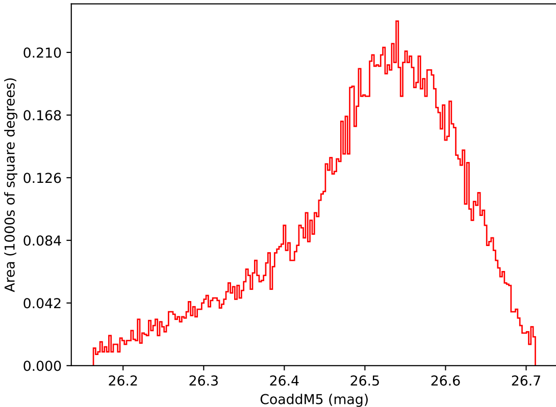
too_elab_r32_d3_ugrizy_v3.4_10yrs WFD i band: CoaddM5
