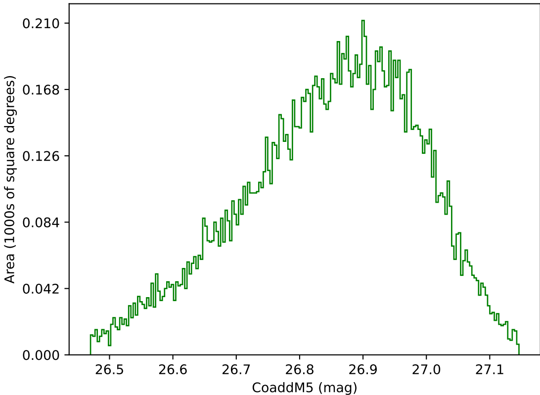
too_elab_r32_d3_ugrizy_v3.4_10yrs WFD g band: CoaddM5
