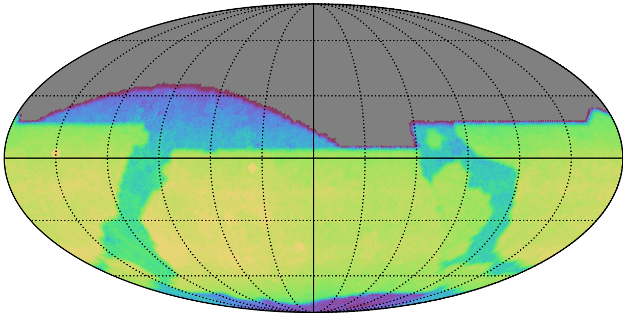
too_elab_r32_d3_ugrizy_v3.4_10yrs All sky z band: CoaddM5
