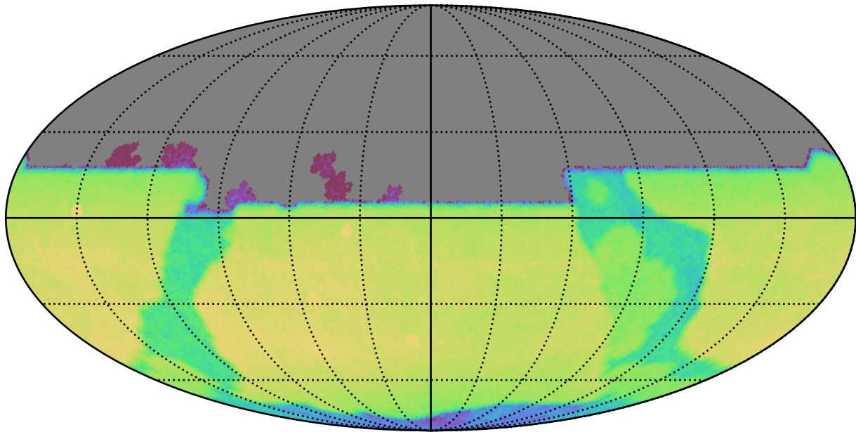
too_elab_r32_d3_ugrizy_v3.4_10yrs All sky y band: CoaddM5
