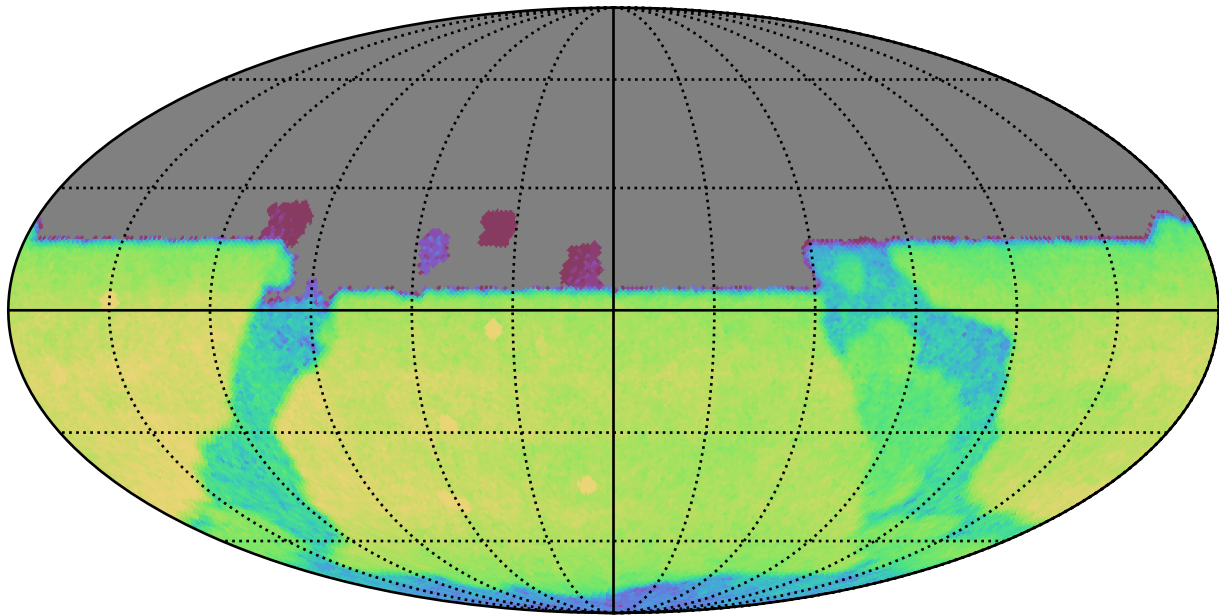
too_elab_r32_d3_ugrizy_v3.4_10yrs All sky u band: CoaddM5
