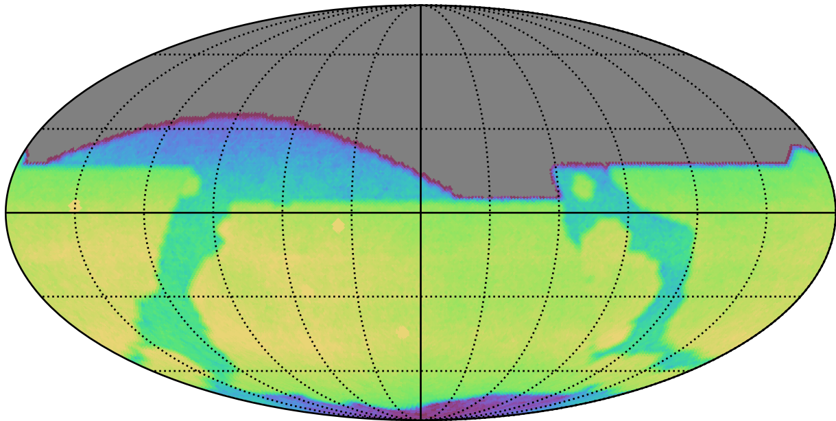
too_elab_r32_d3_ugrizy_v3.4_10yrs All sky r band: CoaddM5
