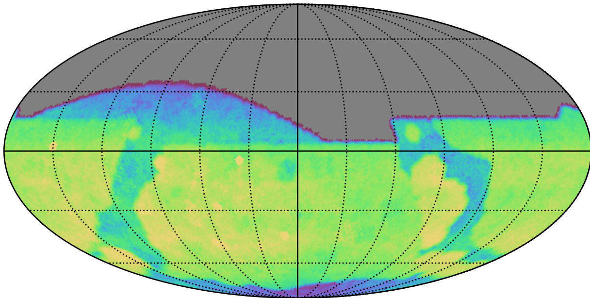
too_elab_r32_d3_ugrizy_v3.4_10yrs All sky g band: CoaddM5
