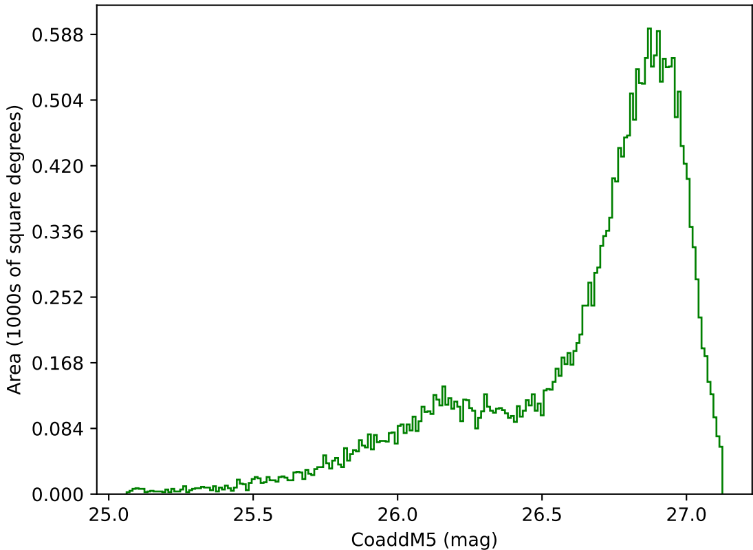
too_elab_r32_d3_ugrizy_v3.4_10yrs All sky g band: CoaddM5
