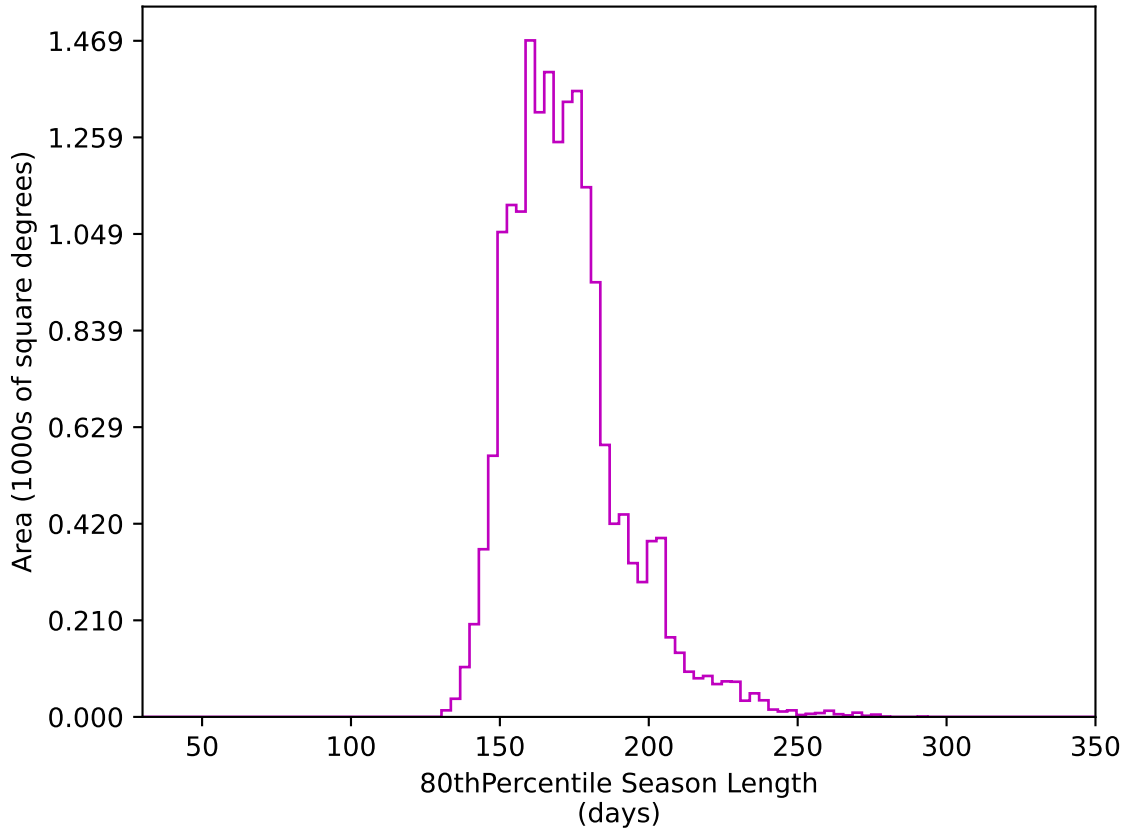
too_elab_r32_d3_ugrizy_v3.4_10yrs WFD z band: 80thPercentile Season Length
