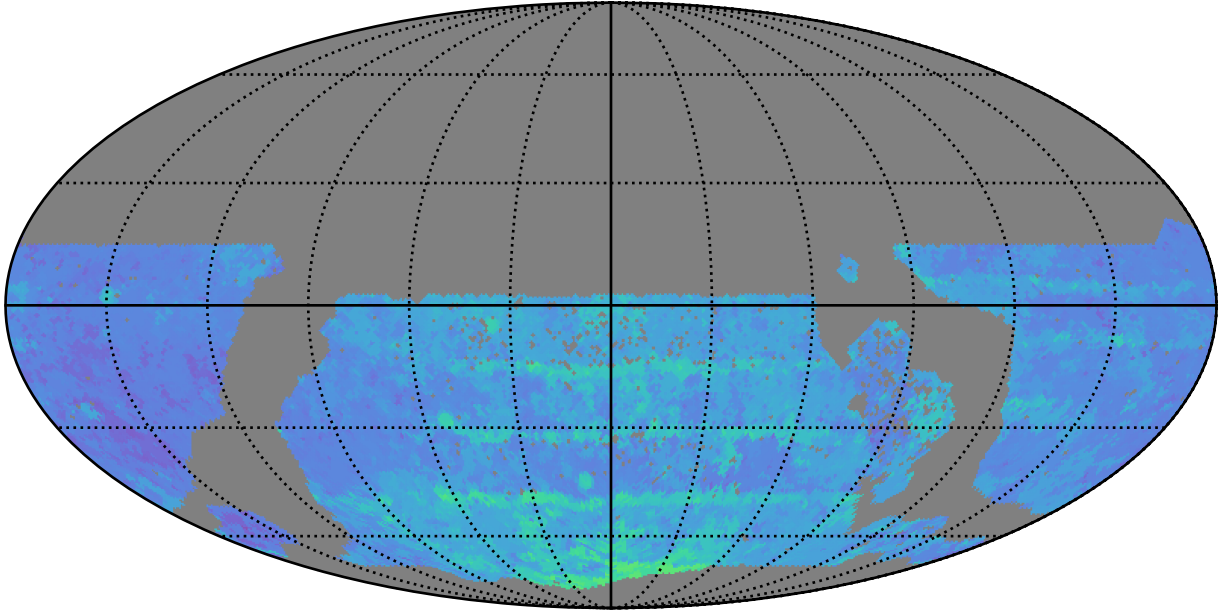
too_elab_r32_d3_ugrizy_v3.4_10yrs WFD y band: 80thPercentile Season Length
