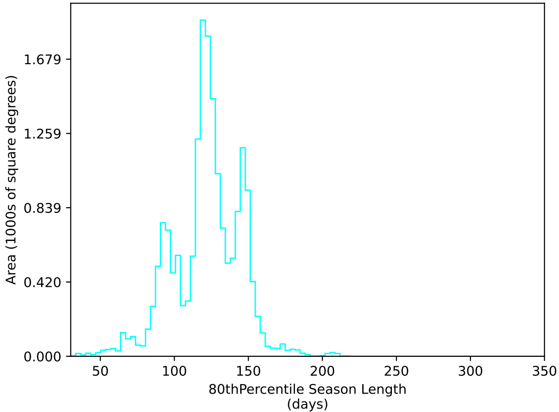
too_elab_r32_d3_ugrizy_v3.4_10yrs WFD u band: 80thPercentile Season Length
