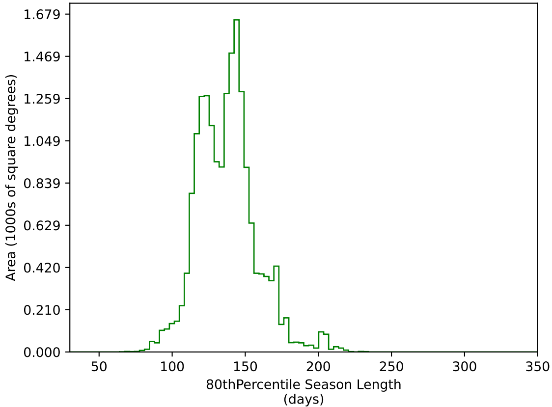
too_elab_r32_d3_ugrizy_v3.4_10yrs WFD g band: 80thPercentile Season Length
