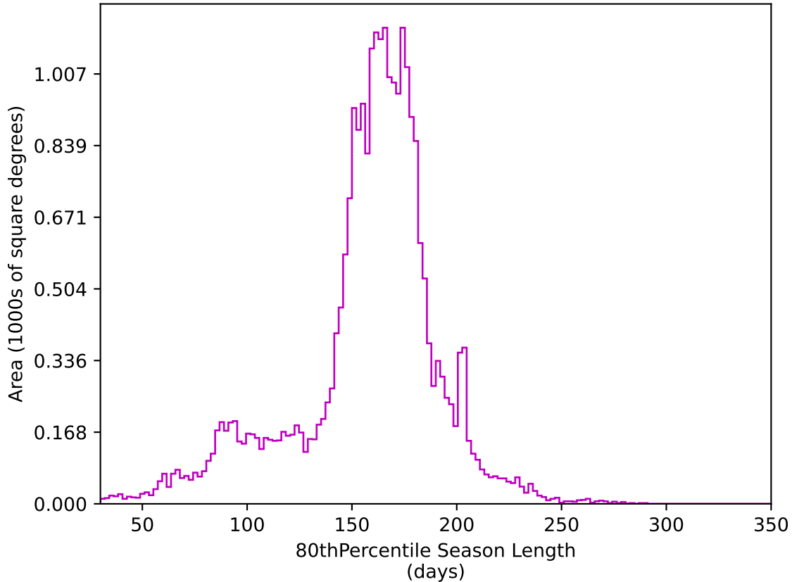
too_elab_r32_d3_ugrizy_v3.4_10yrs All sky z band: 80thPercentile Season Length
