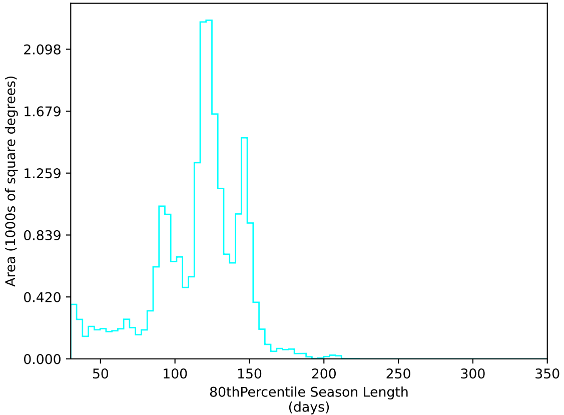
too_elab_r32_d3_ugrizyv3.4_10yrs All sky u band: 80thPercentile Season Length
