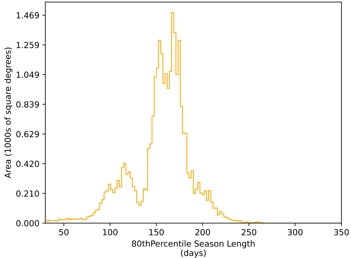
too_elab_r32_d3_ugrizy_v3.4_10yrs All sky r band: 80thPercentile Season Length
