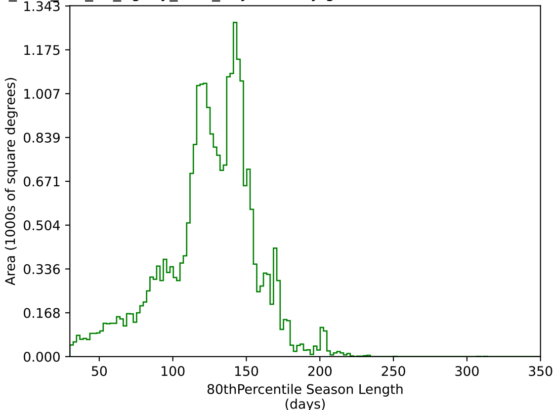
too_elab_r32_d3_ugrizy_v3.4_10yrs All sky g band: 80thPercentile Season Length
