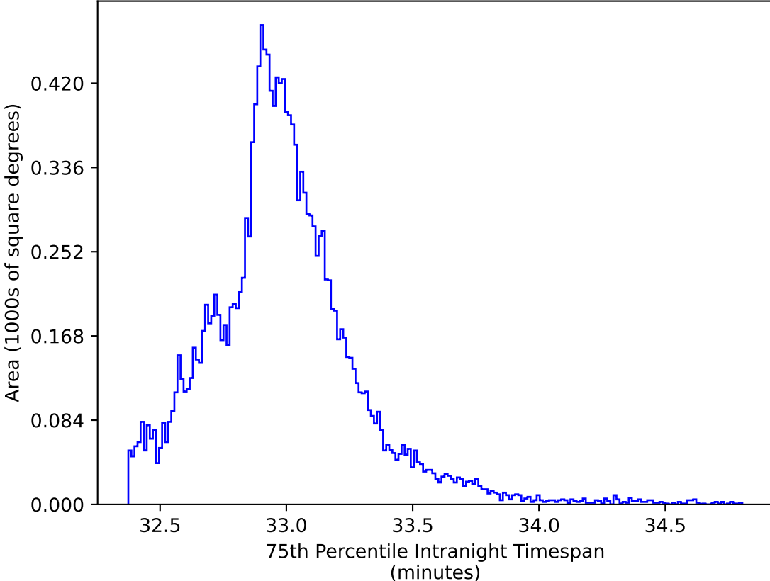
too_elab_r32_d3_ugrizy_v3.4_10yrs WFD y band: 75th Percentile Intranight Timespan
