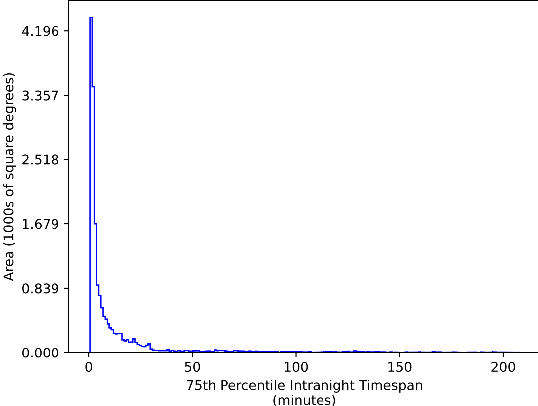
too_elab_r32_d3_ugrizy_v3.4_10yrs WFD u band: 75th Percentile Intranight Timespan
