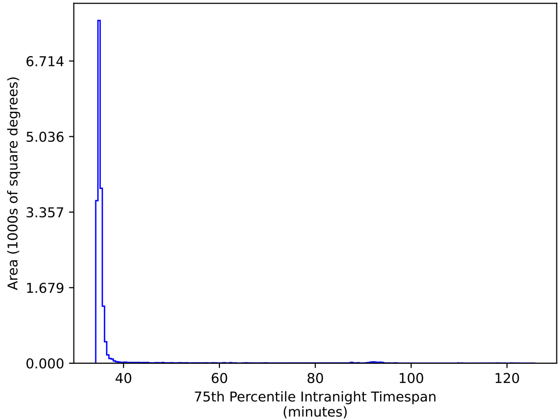
too_elab_r32_d3_ugrizy_v3.4_10yrs WFD ri bands: 75th Percentile Intranight Timespan
