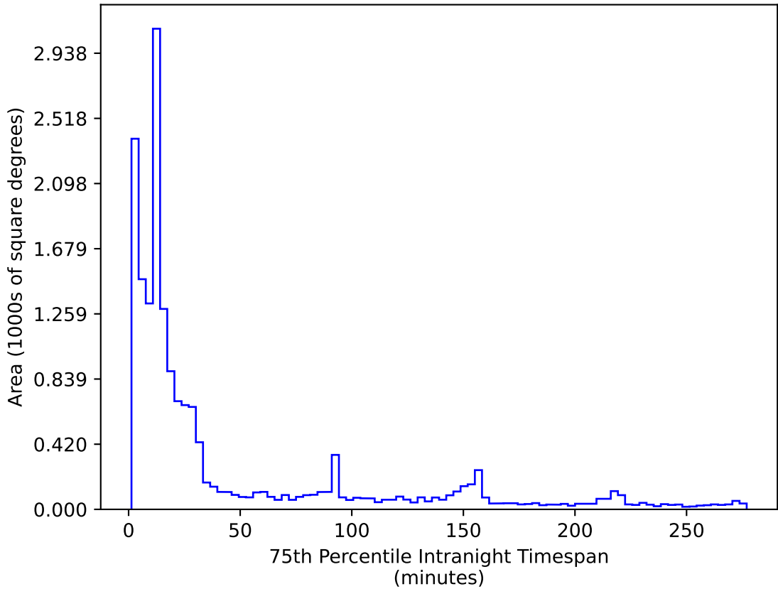
too_elab_r32_d3_ugrizy_v3.4_10yrs WFD r band: 75th Percentile Intranight Timespan
