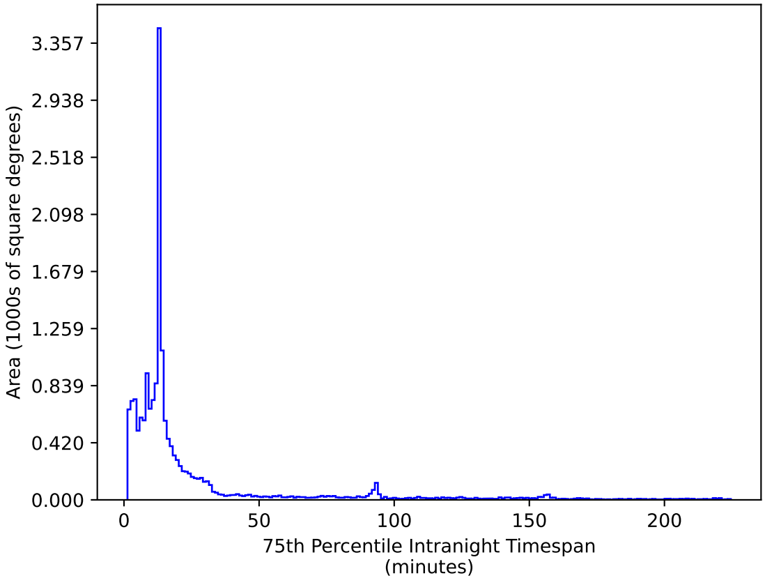
too_elab_r32_d3_ugrizy_v3.4_10yrs WFD i band: 75th Percentile Intranight Timespan
