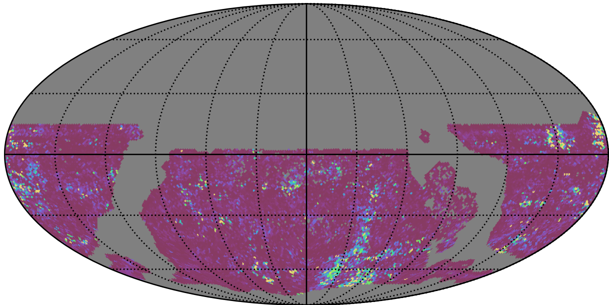
too_elab_r32_d3_ugrizy_v3.4_10yrs WFD g band: 75th Percentile Intranight Timespan
